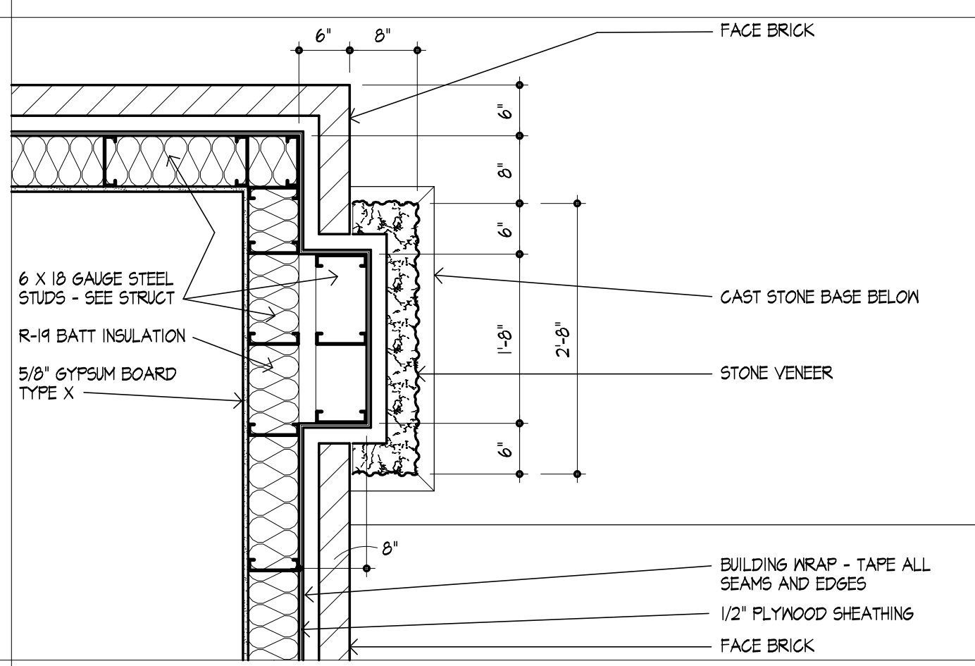
1 DETAIL SCALE 3/4" = 1'-0"
