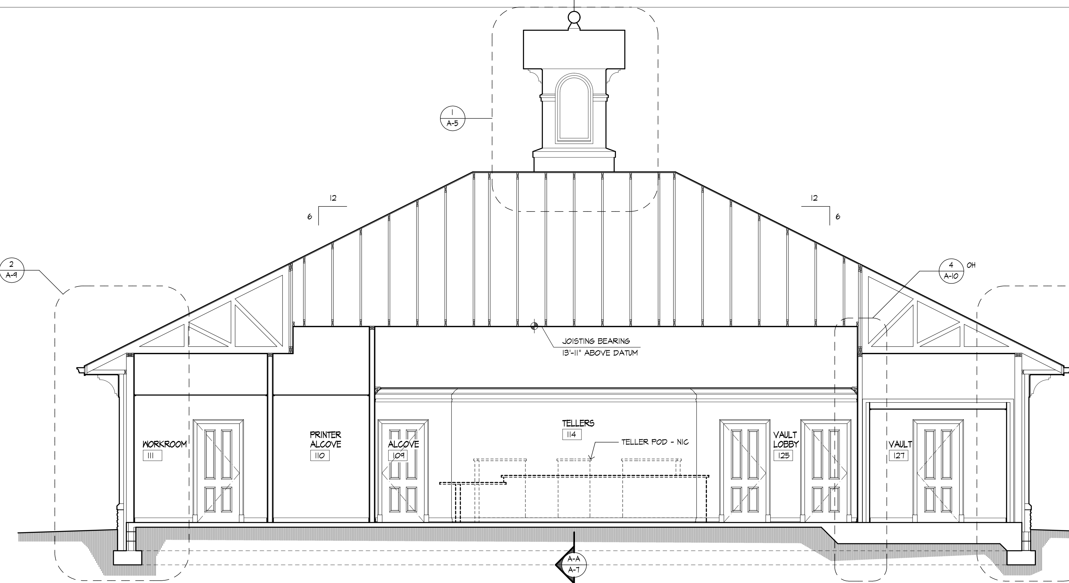
BUILDING SECTION B-B SCALE 1/4" = 1'-0"
