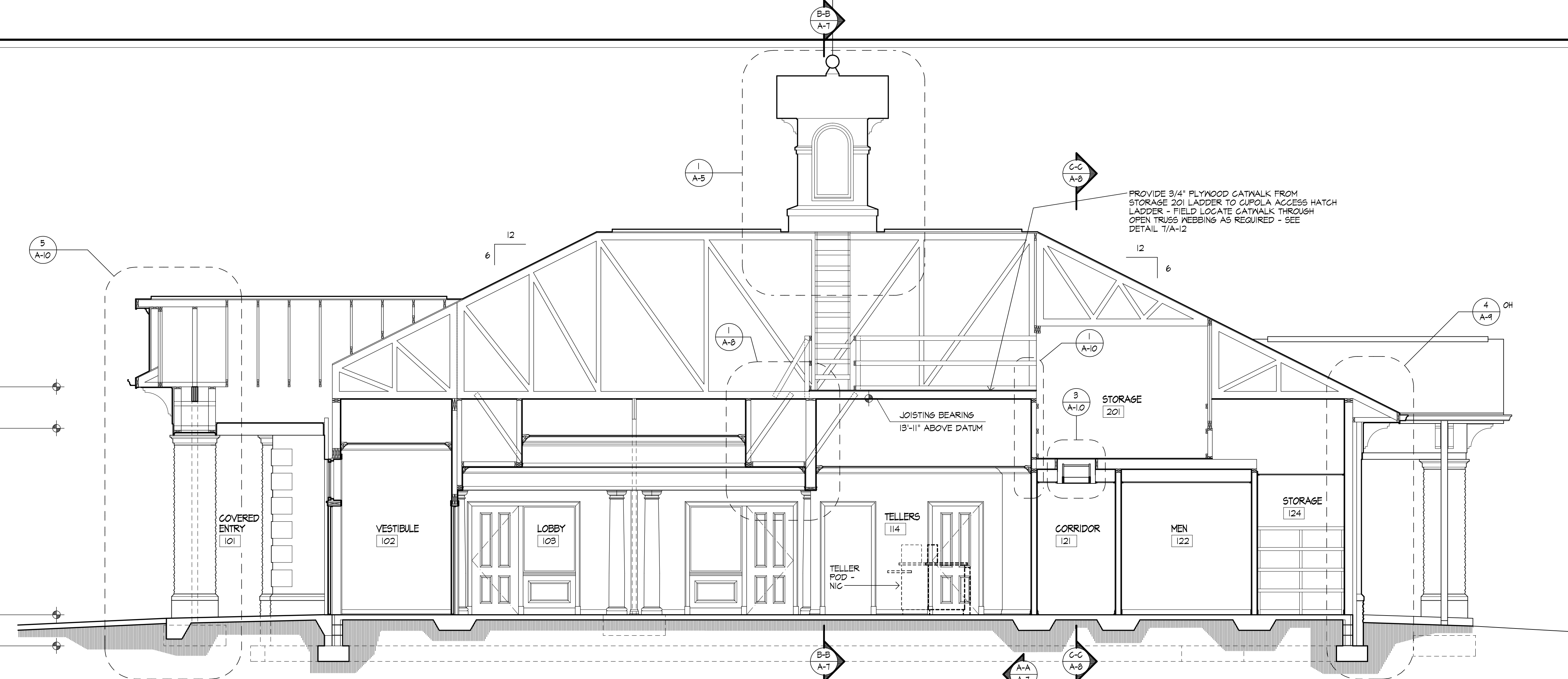
BUILDING SECTION A-A SCALE 1/4" = 1'-0"
