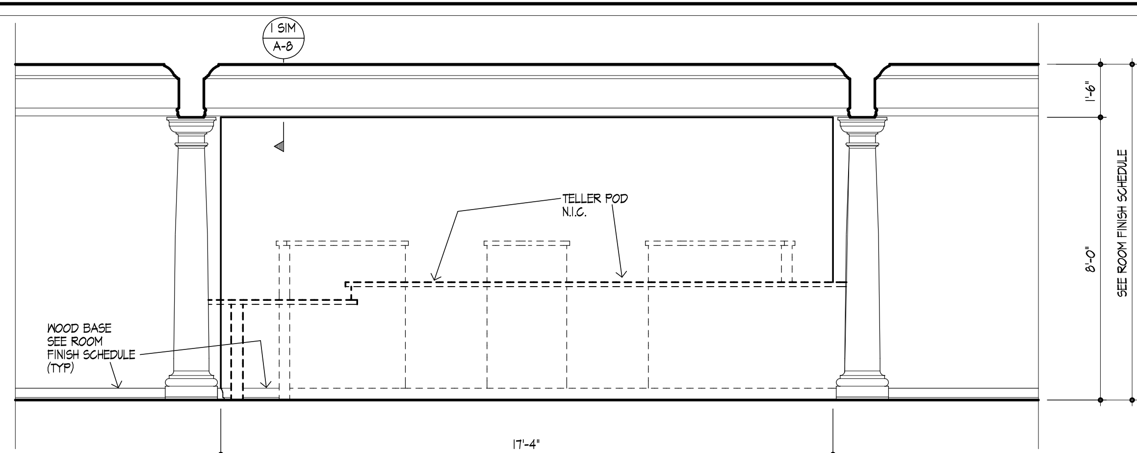
1 ELEVATION TELLERS 114
