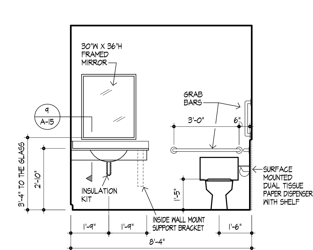
12 ELEVATION MEN 122 & WOMEN 120 OPPOSITE HAND
