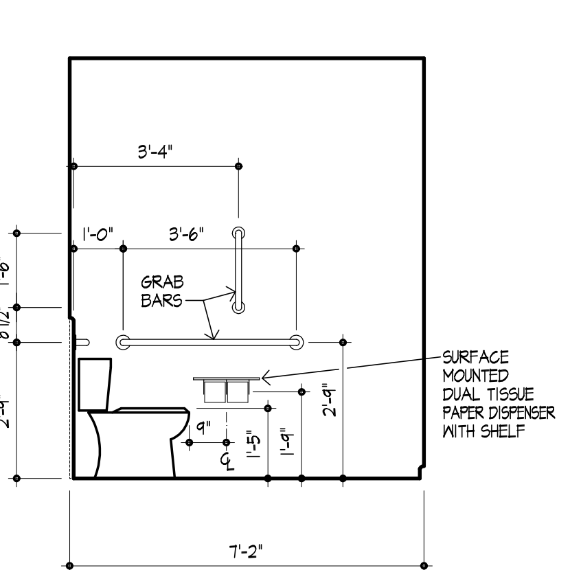
13 ELEVATION MEN 122 & WOMEN 120 OPPOSITE HAND
