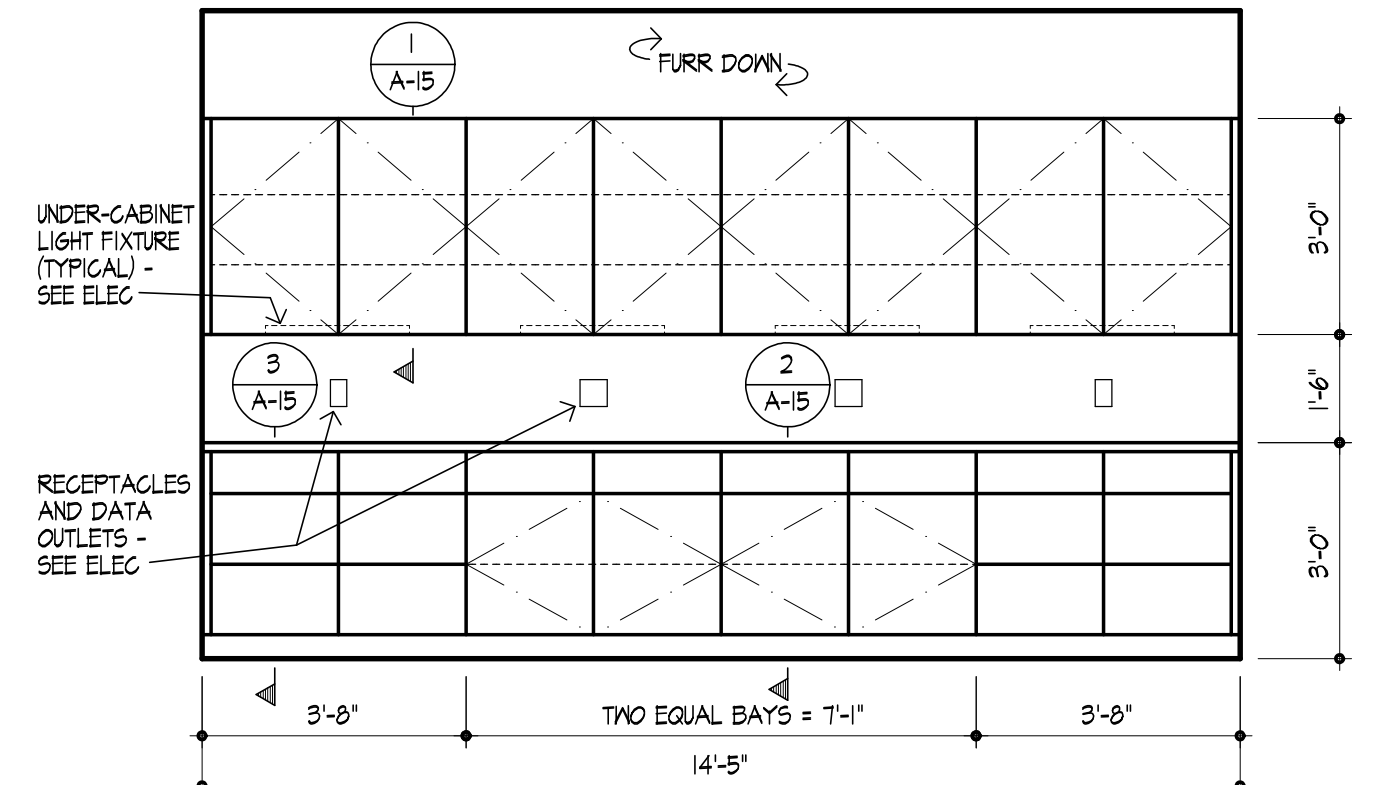
6 ELEVATION WORKROOM 111
