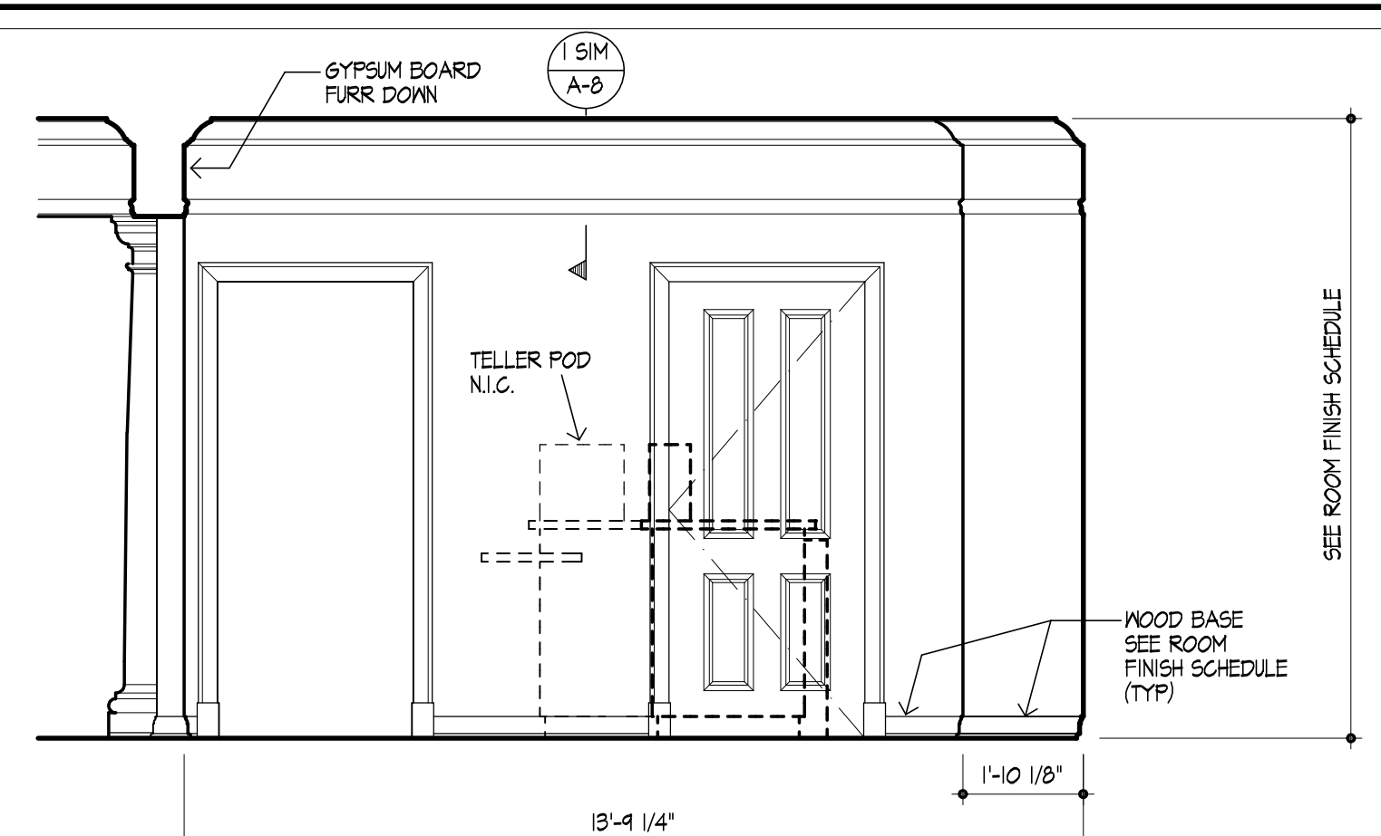
3 ELEVATION TELLERS 114
