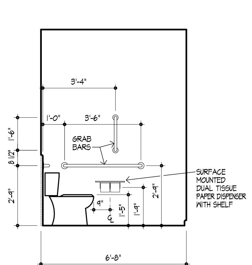
8 ELEVATION TOILET 113
