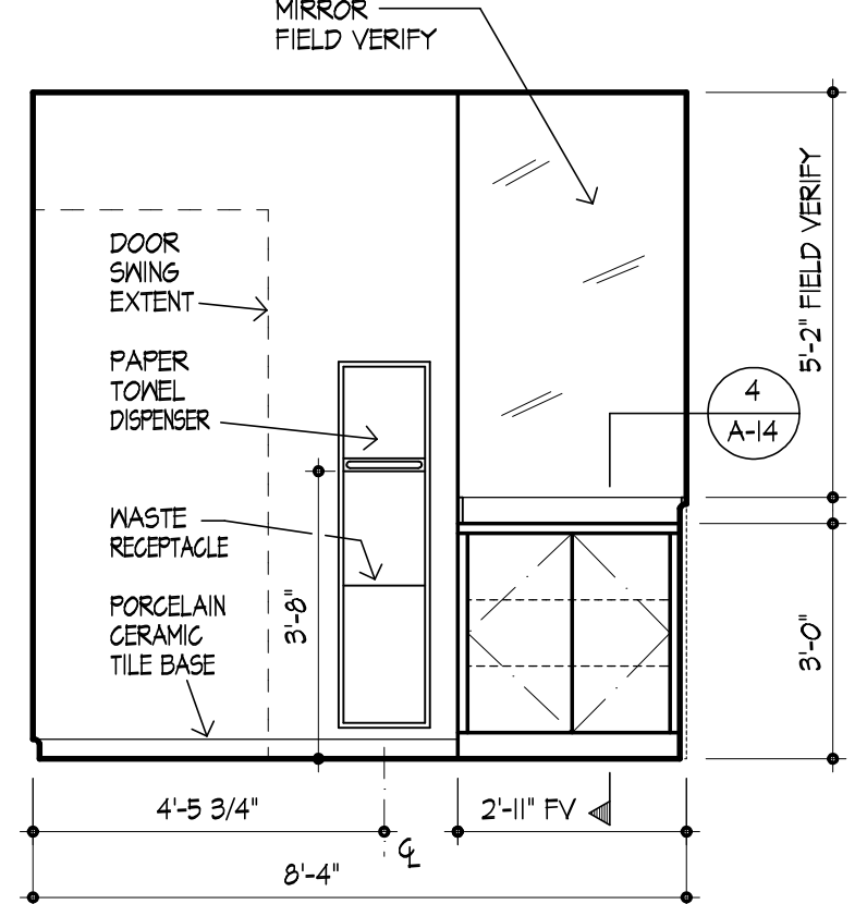
15 ELEVATION WOMEN 120
