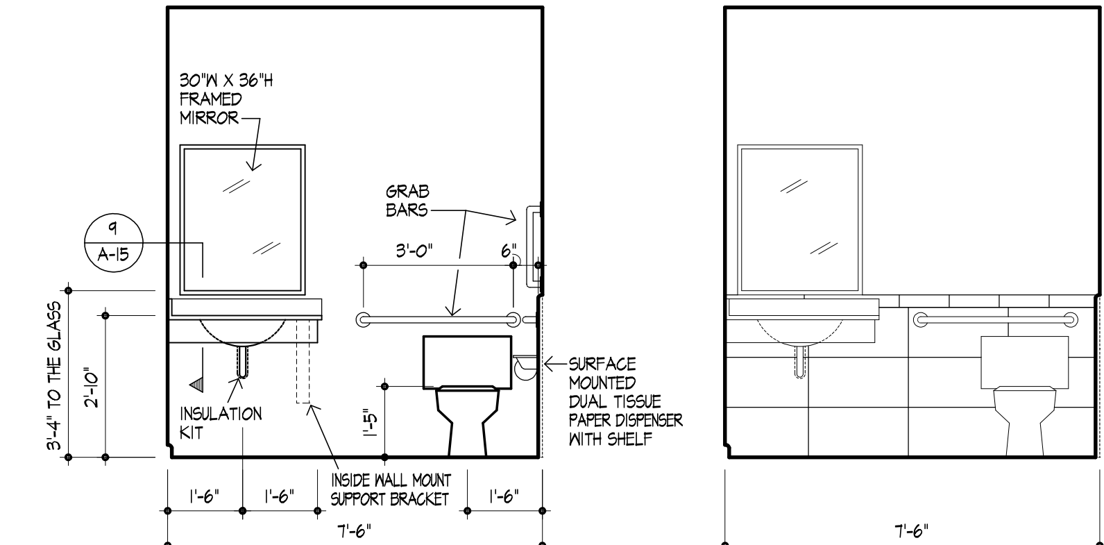
7 ELEVATION TOILET 113
