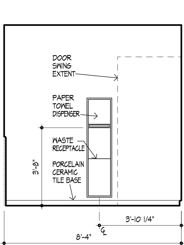
14 ELEVATION MEN 122
