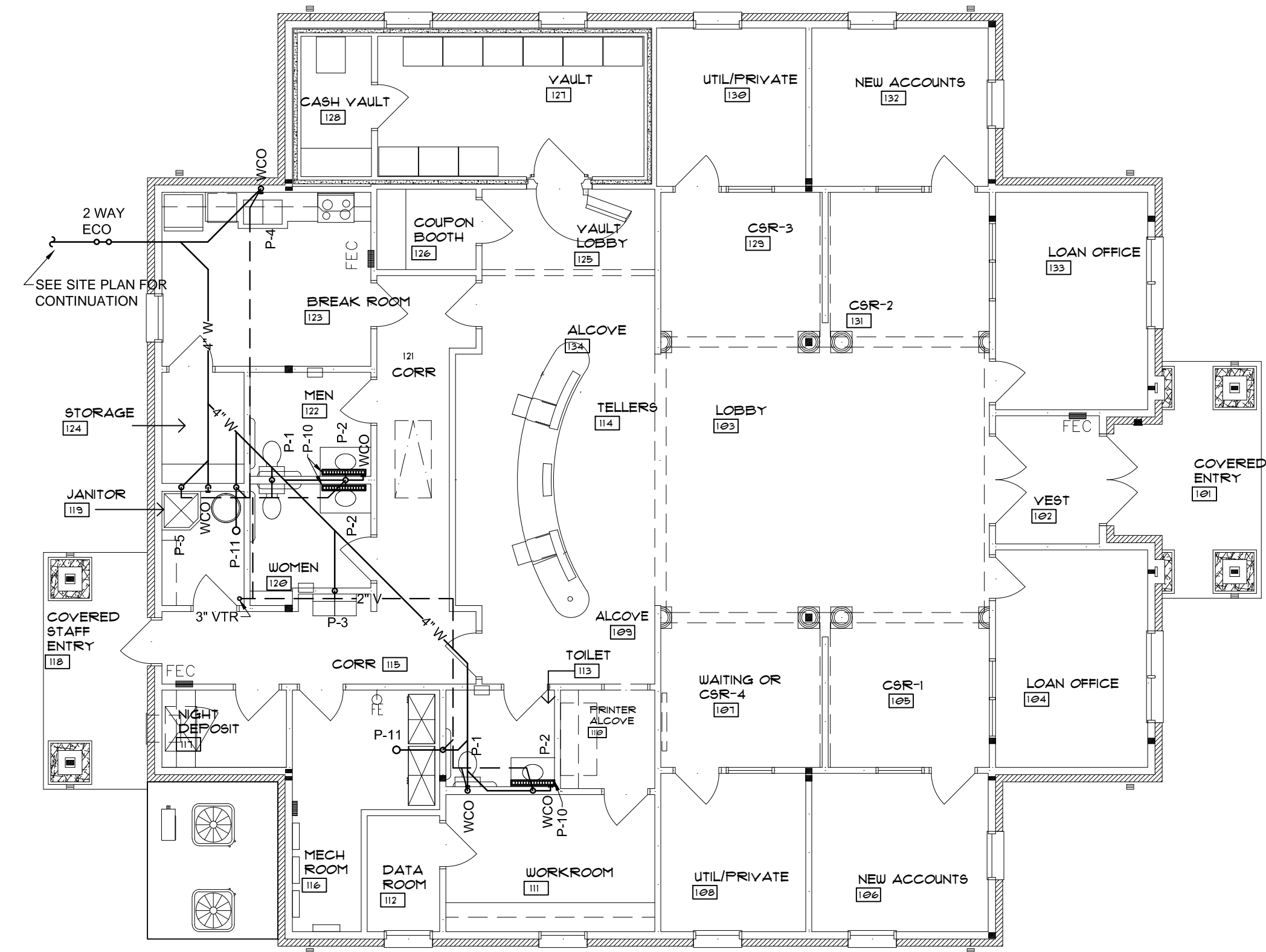
NEW CONSTRUCTION - WASTE AND VENT PLUMBING FLOOR PLAN SCALE: 1/8" = 1'-0"
